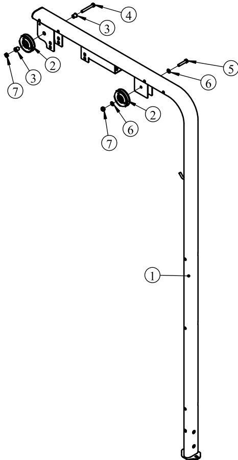
Left Standing Frame II ASSY
